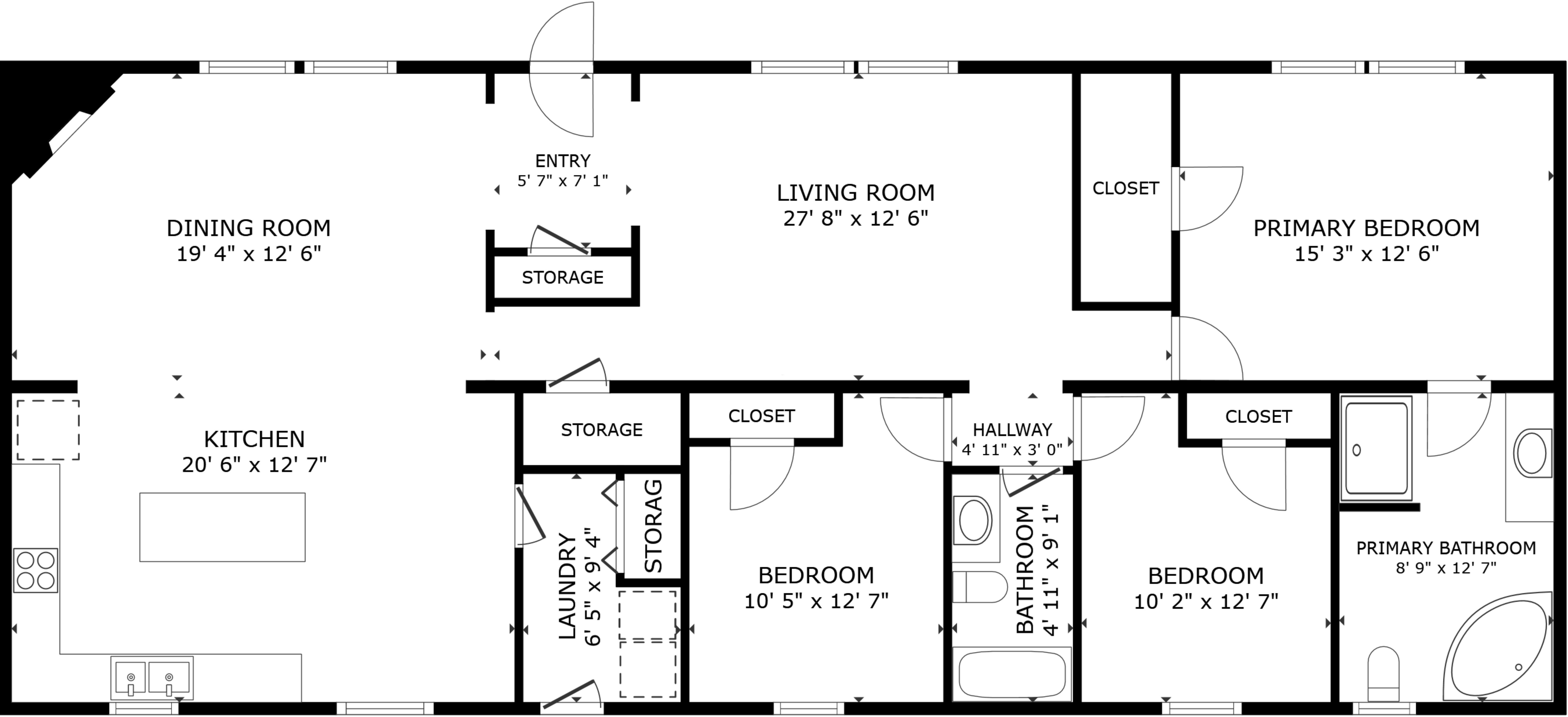
FLOOR PLAN
